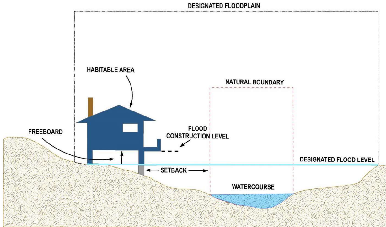
Figure 9 – Floodplain Illustration
